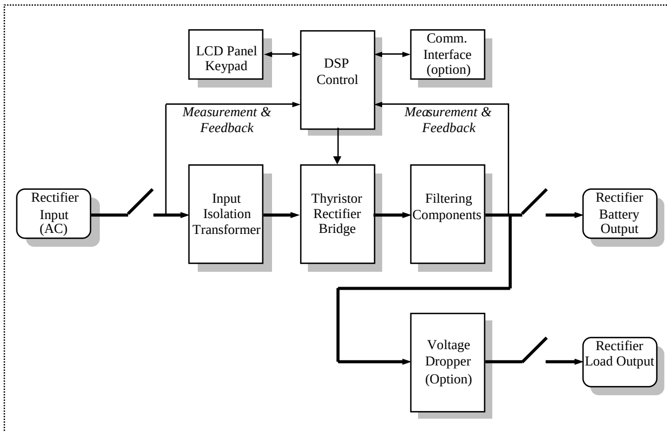
AETES XTM Series Industrial SCR Rectifier/Charger Block Diagram
